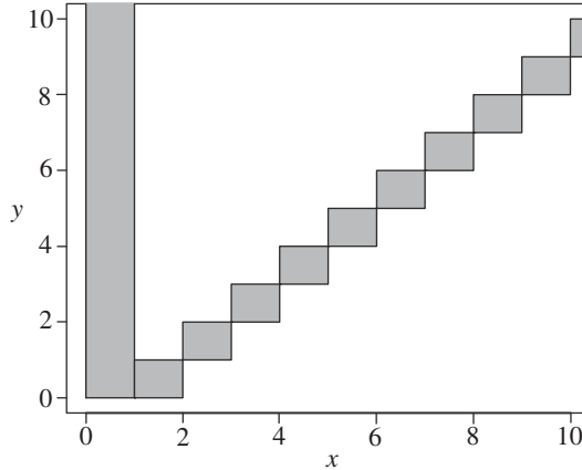
FIGURE 1: The region A used in the proof of Proposition 3.
