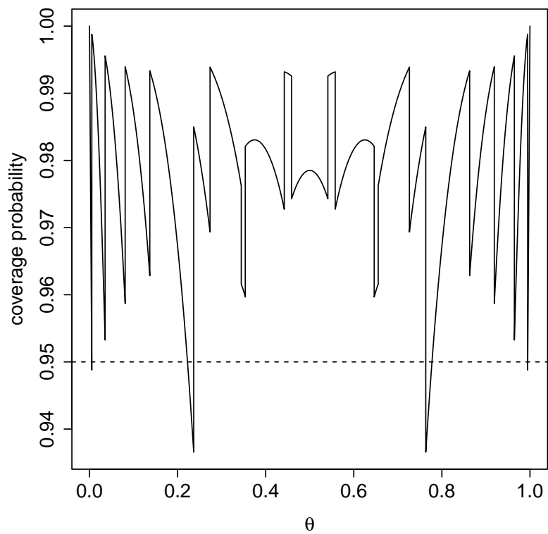
Figure 1: Coverage probability of the nominal 95% confidence interval for the binomial distribution with sample size n = 10 calculated by the function prop.test in the R statistical computing language (Ihaka and Gentleman, 1996). This is the Wilson (also called, score) interval with continuity correction and modifications when x = 0 or x = n . The dashed line is the nominal level. The solid line is the coverage probability of the interval as a function of the success probability \theta .
