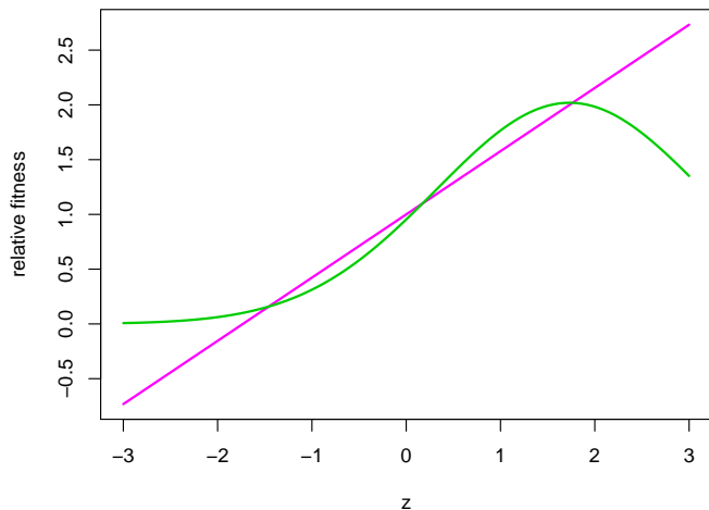
Figure: Fitness landscape (green) and its best quadratic approximation (magenta). \sigma^2 = 1 , \lambda = 2 , \eta = \sqrt{\lambda + \sigma^2} = 1.732 .
