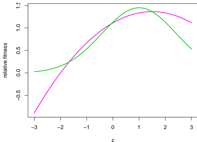
Figure: Fitness landscape (green) and its best quadratic approximation (magenta). \sigma^2 = 1 , \lambda = 2 , \eta = 1
